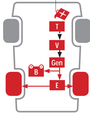
Serieller Hybrid
